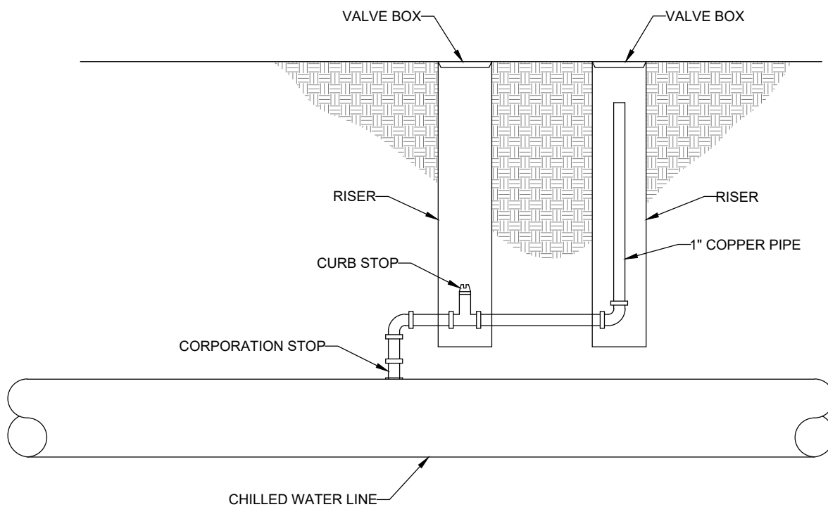
1 AIR RELEASE VALVE DETAIL M1.01 SCALE: NO SCALE
