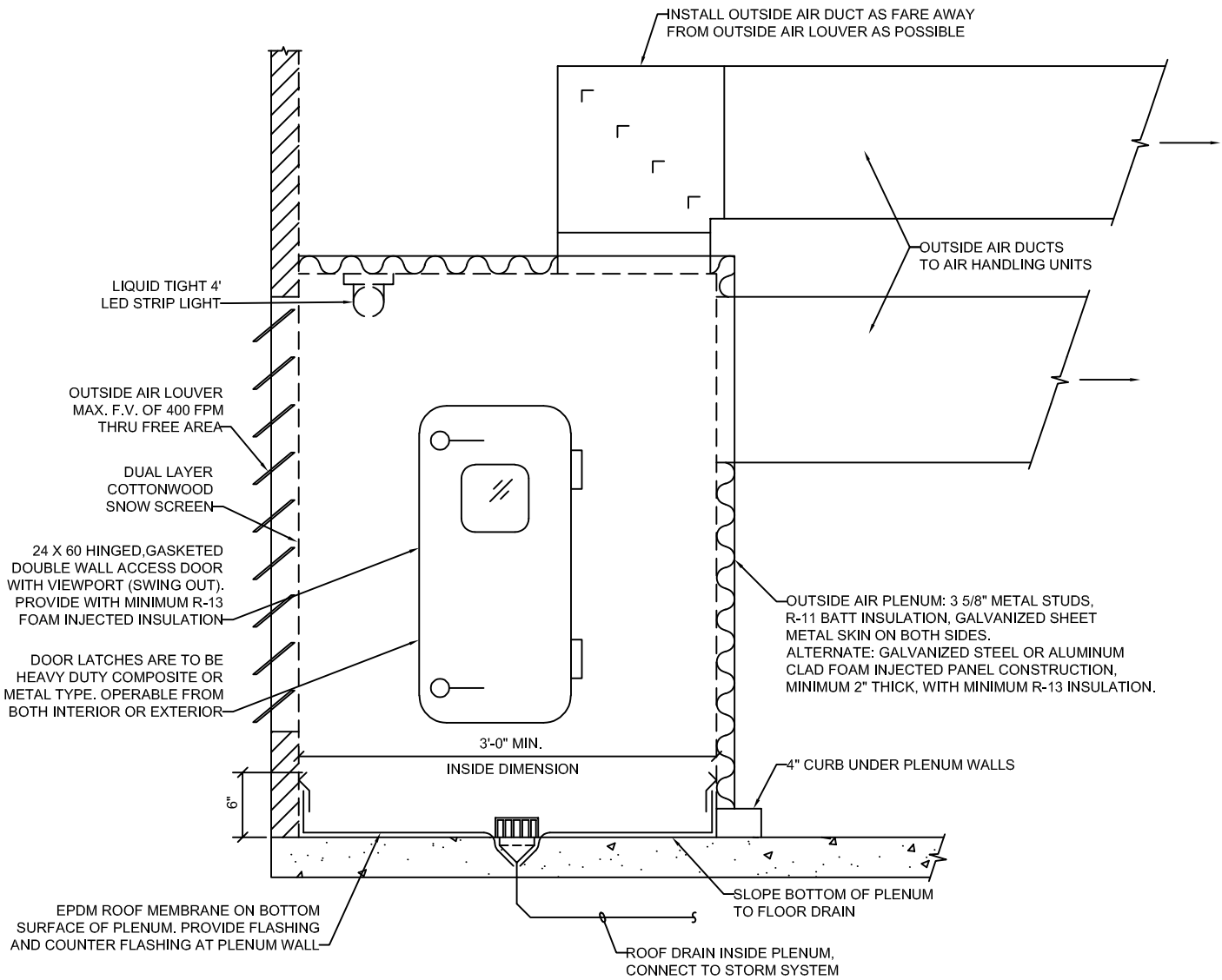
1 OUTSIDE AIR PLEMUM DETAIL A1.01 SCALE: NO SCALE
