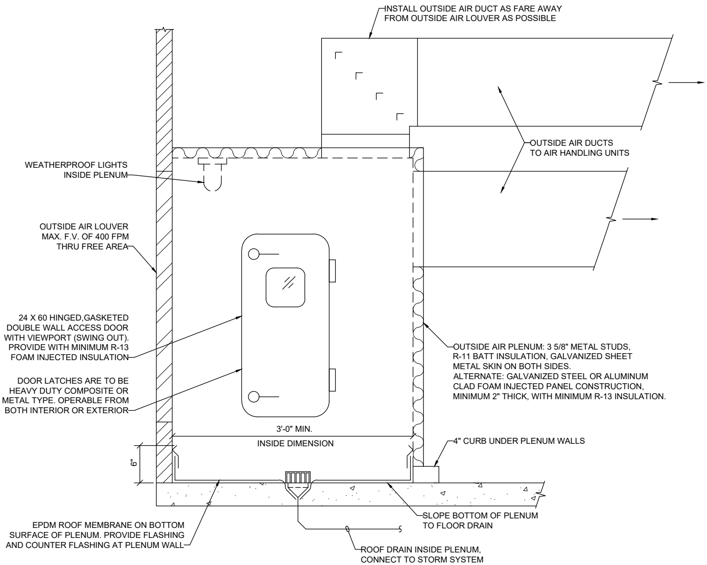
1 OUTSIDE AIR PLENUM DETAIL A1.01 SCALE: NO SCALE
