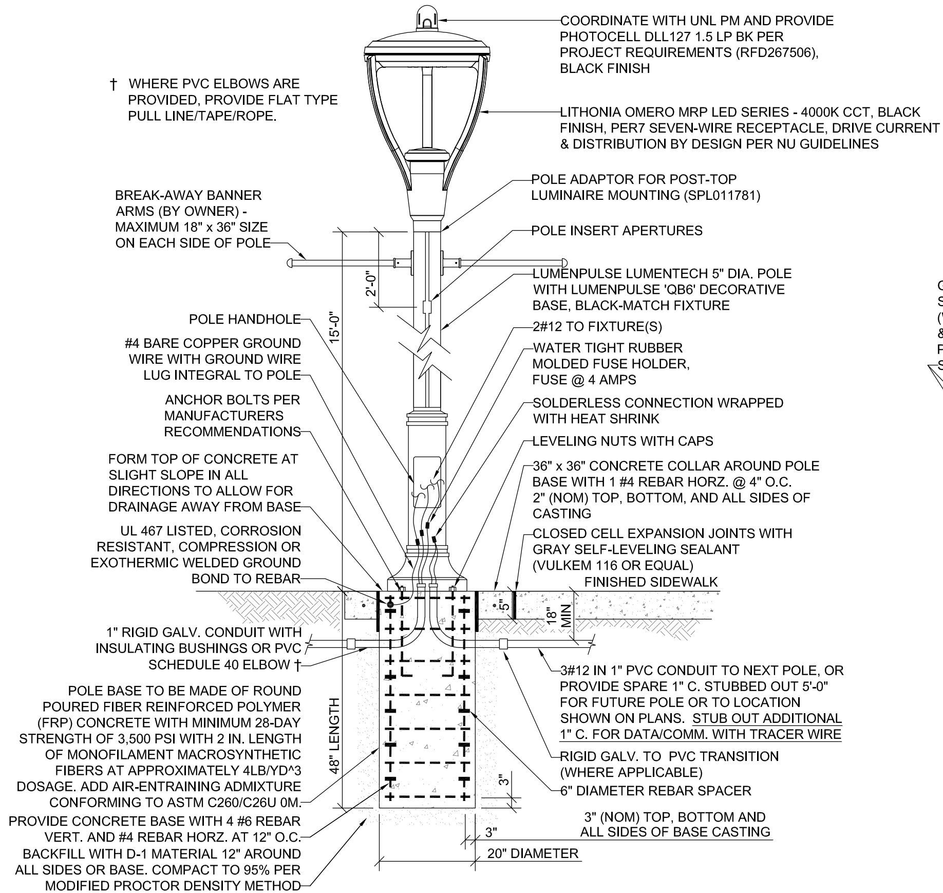
1 PEDESTRIAN POLE 'B' DETAIL E1.01 SCALE: NO SCALE
