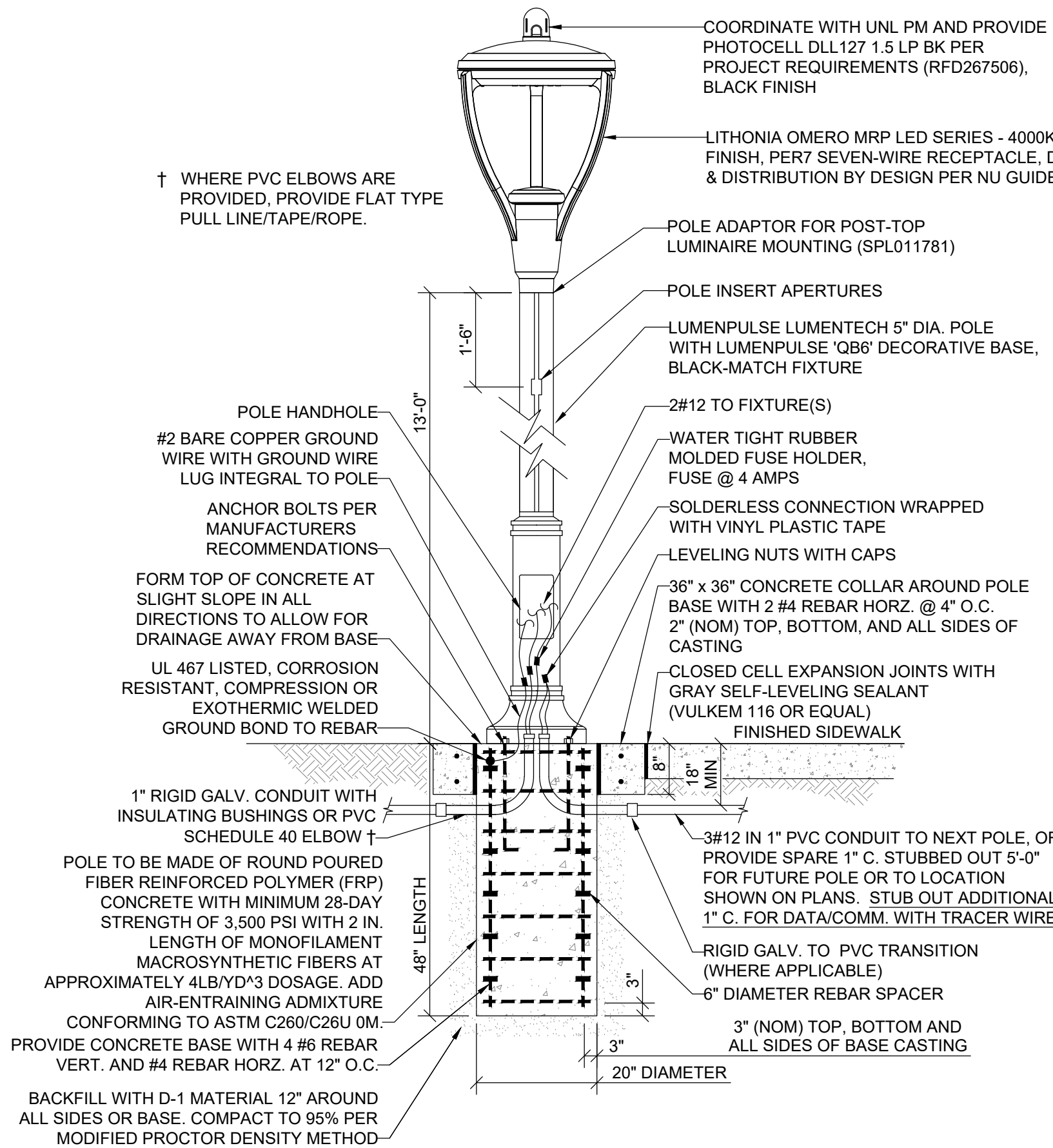
1 PEDESTRIAN POLE 'A' DETAIL E1.01 SCALE: NO SCALE
